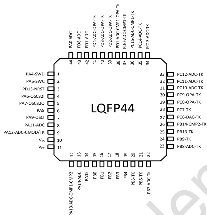
图 3-3 LQFP44 Pinout1 PY32T090S1xT7 (Top view)
