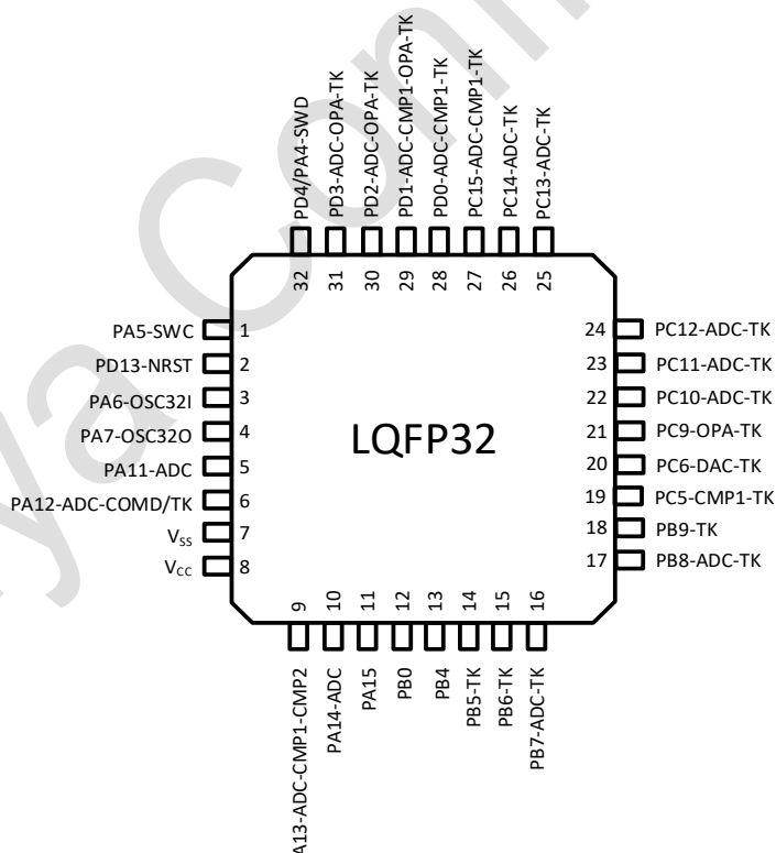
图 3-4 LQFP32 Pinout1 PY32T090K1xT7 (Top view)
